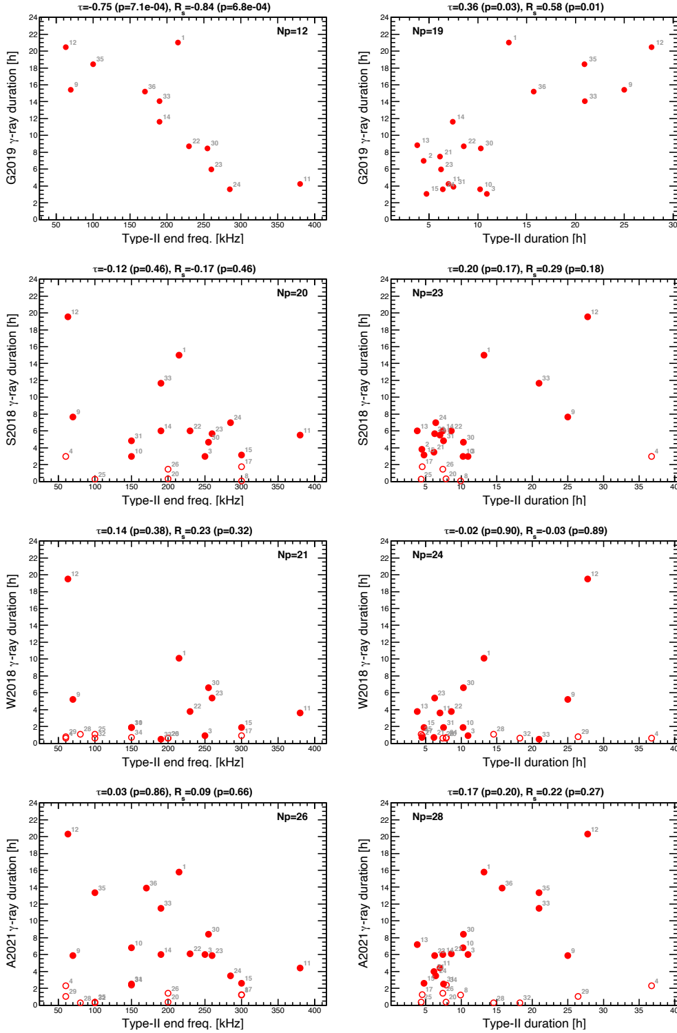
Figure 6. Scatter plots of the LDGRF duration as a function of the type-II end frequency (left panels) and duration (right panels). From top to bottom: the calculation using results from Gopalswamy et al. (2019, G2019), Share et al. (2018, S2018), Winter et al. (2018, W2018) and Ajello et al. (2021, A2021). The number of events used in each plot, along with the Kendall ( \tau ) and Spearman ( R_s ) correlation coefficients (and corresponding p-values) are reported for each panel. The event numbers in Table 3 are printed adjacent to the data points. The empty markers indicate events not included by Gopalswamy et al. (2019).
