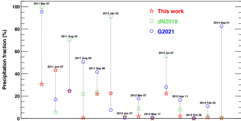
Figure 3. Comparison between the precipitation fraction lower limits derived in this work, using the N_{SEP} upper limits based on the CME latitudes from Gopalswamy et al. (2014), and the precipitation fractions estimated by de Nolfo et al. (2019, dN2019) and Gopalswamy et al. (2021, G2021). All the calculations rely on the N_{LDGRF} values from Share et al. (2018). The dotted lines are to guide the eye.
