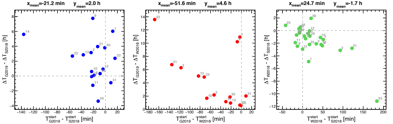
Figure 5. Scatter plots of the difference between the \gamma -ray event durations \Delta T vs the difference between the corresponding onset times T^{\text{start}} , based on the estimates from Gopalswamy et al. (2019, G2019) , Share et al. (2018, S2018) and Winter et al. (2018, W2018) . The event numbers in Table 3 are printed adjacent to the data points.
