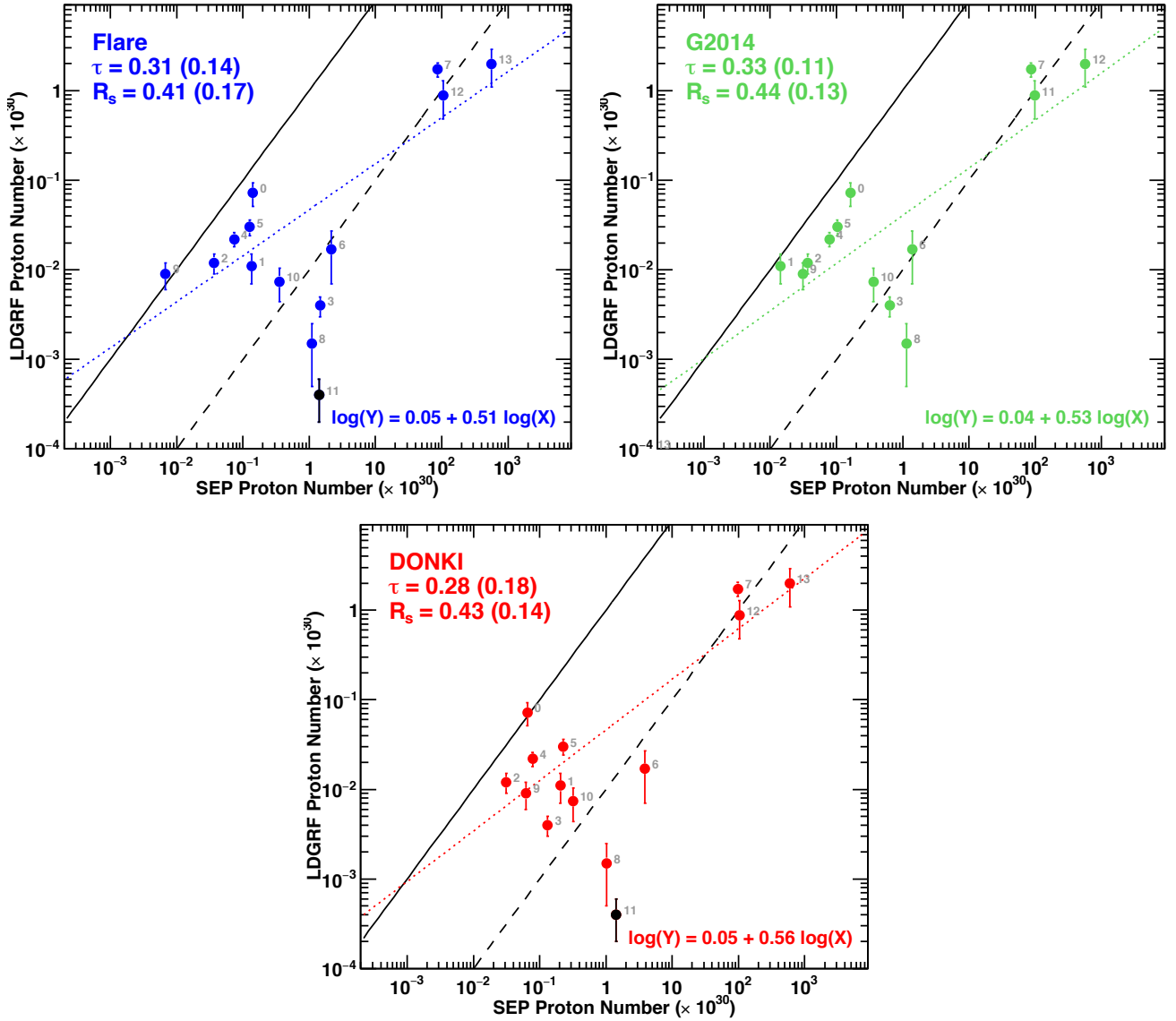
Figure 1. Scatter plots of the N_{LDGRF} vs N_{SEP} values obtained by using the upper limits on the numbers of >500 MeV interplanetary protons. The three panels report the calculations made implementing the flare latitudes (blue, top left panel) and the CME latitudinal angles from Gopalswamy et al. (2014, G2014) (green, top right panel) and DONKI (red, bottom panel) – see Table 1 , with corresponding Kendall ( \tau ) and Spearman ( R_s ) correlation factors and relative p-values between brackets. The event numbers in Table 1 are printed adjacent to the data points. The colored dotted lines indicates the corresponding bi-logarithmic regression lines, with parameters reported in the bottom-right corners. The solid and dashed black lines mark the 1-to-1 and the 1-to-100 correspondences, respectively. The black point marks the 2013 October 28 event, not included in the correlation and the regression estimates.
