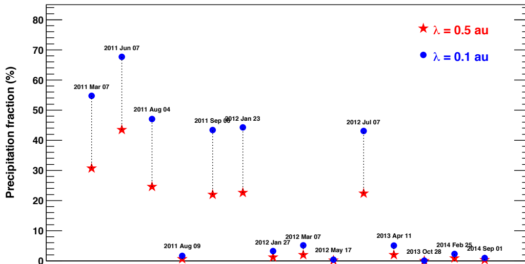
Figure 4. Comparison between the precipitation fraction lower limits using the different interplanetary turbulence conditions, as parameterized by the mean free path \lambda . Both calculations are based on the N_{SEP} upper limits obtained with the CME latitudes from Gopalswamy et al. (2014) and the N_{LDGRF} values from Share et al. (2018) .
